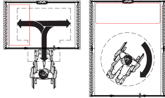
Clear floor space
