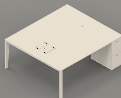
W 1400 / 1600 / 1800 / 2000 x D 1200 / 1400 / 1600 x H 740 mm BENCH WITH SUPPORT PEDESTAL BENCH AVEC CAISSON SUPPORT BENCH CON BLOQUE SOPORTE BENCH COM BLOCO SUPORTE
